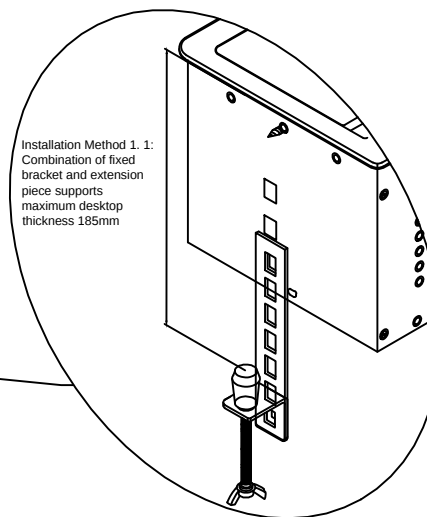
Installation method
